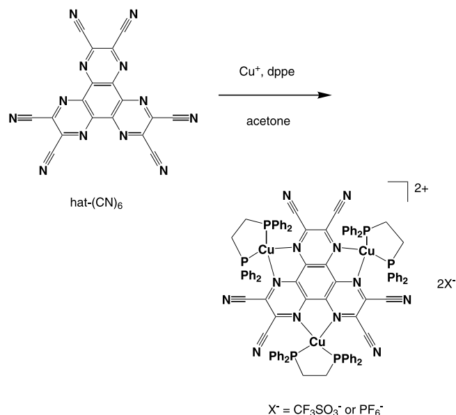
Fig. 5. Synthesis of [\{\text{Cu}(\text{dppe})\}_3\{\text{hat}-(\text{CN})_6\}]^{2+} . The complex contains stable radical anion, [\text{hat}-(\text{CN})_6]^- , coordinating to three copper(I) ions.
