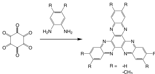
Fig. 4. Syntheses of hat and its derivatives.
