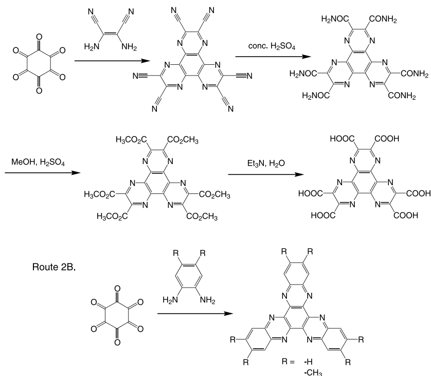
Fig. 4. Syntheses of hat and its derivatives.
