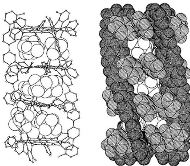
Fig. 8. Crystal structure of [\text{Cu}_{12}(\text{octapy})_3\{\text{hat}-(\text{Ph})_6\}_4]^{12+} . The structure is schematically represented as an analogue of 3d type in Fig. 3 (original Figure 5 from Ref. [21]).
