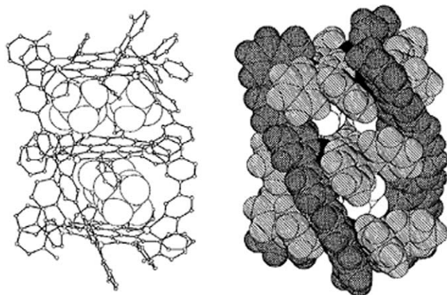
Fig. 7. Crystal structure of [\text{Cu}_9(\text{spy})_3\{\text{hat}-(\text{Ph})_6\}_3]^{9+} . The structure is schematically represented as an analogue of 3d type in Fig. 3 (original Figure 4 from Ref. [21]).
