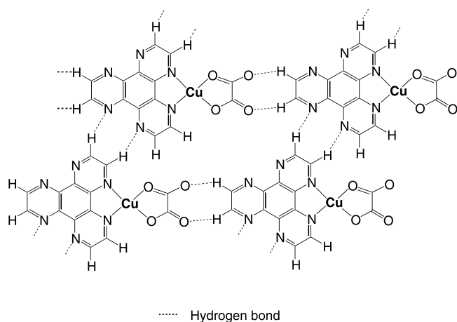
Fig. 16. Hydrogen bond-linked network within the sheet.
