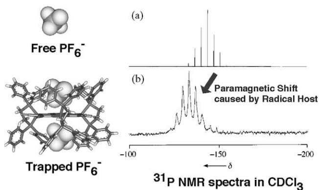
Fig. 27. ^{31}P -NMR spectra at room temperature for nBu_4NPF_6 (a) and [Cu(dppe)_3\{hat-(CN)_6\}](PF_6)_2 (b) in CDCl_3 solution.
