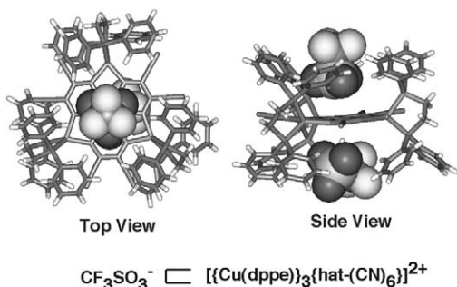
Fig. 26. Anion trap structure of [Cu(dppe)_3\{hat-(CN)_6\}](CF_3SO_3)_2 .
